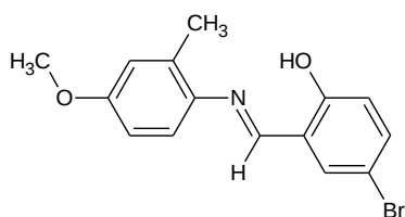
Fig. 1 Primary ligand 4-bromo-2-{(E)-[(4-methoxy-2-methylphenyl)imino]methyl}phenol
