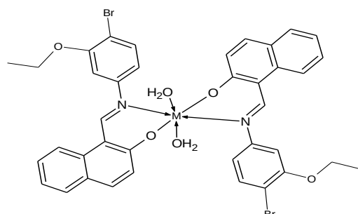
Fig. 3 The metal-ligand binary binding proposed structure
