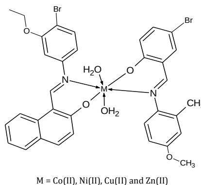
Fig. 4 The metal-ligand ternary binding proposed structure
